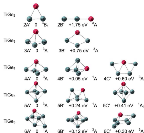
Fig. 4 Optimized geometries of the low-lying isomers of \text{TiGe}_n^- ( n = 2-6 ) clusters. The relative energies to the most stable isomers (on the left) are shown.
