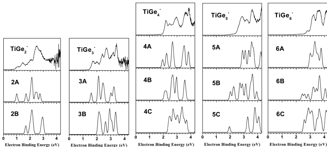
Fig. 3 Comparison between the experimental photoelectron spectra and simulated DOS spectra of the low-lying isomers of \text{TiGe}_n^- ( n = 2-6 ) clusters. The simulations were conducted by fitting the distribution of the transition lines with unit-area Gaussian functions of 0.15 eV FWHM.
