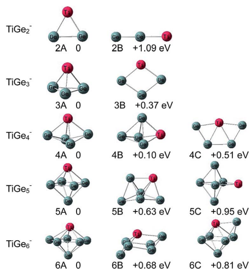
Fig. 2 Optimized geometries of the low-lying isomers of \text{TiGe}_n^- ( n = 2-6 ) clusters. The relative energies to the most stable isomers (on the left) are shown.
