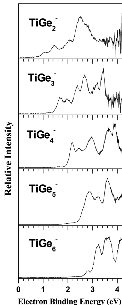
Fig. 1 Photoelectron spectra of \text{TiGe}_n^- ( n = 2-6 ) clusters recorded with 266 nm photons.
