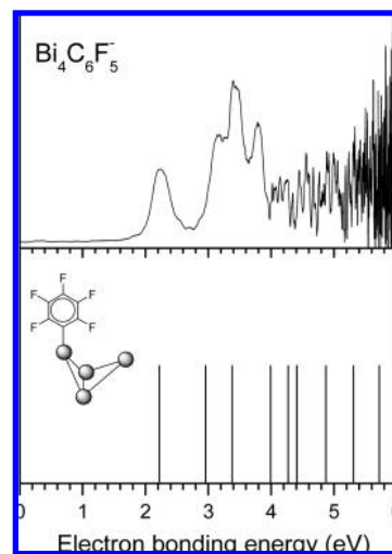
Figure 14. The comparison of PE spectrum of Bi_4C_6F_5^- with the simulated spectrum based on Koopmans' theorem for isomer 4a of Bi_4C_6F_5^- .
