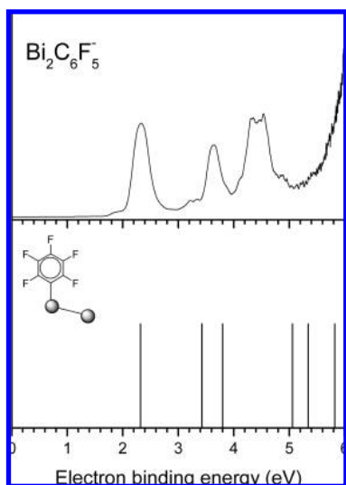
Figure 12. The comparison of PE spectrum of Bi_2C_6F_5^- with the simulated spectrum based on Koopmans' theorem for isomer 2a of Bi_2C_6F_5^- .
