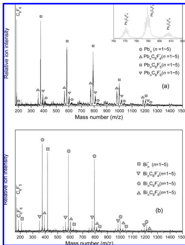
Figure 1. Typical mass spectra of the anionic products from the reactions between metal ( \text{M} = (a) Pb and (b) Bi) by laser ablation and hexafluorobenzene seeded in argon carrier gas (0.1% hexafluorobenzene in 400 kPa mixed gas). The inset in Figure 1a shows the enlarged part of the spectrum.
