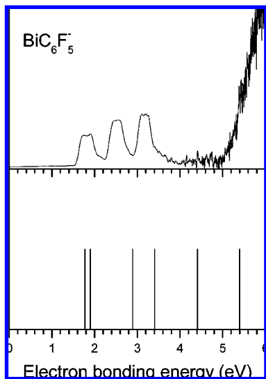
Figure 11. The comparison of PE spectrum of BiC_6F_5^- with the simulated spectrum based on Koopmans' theorem for the optimized ground state structure of BiC_6F_5^- .
