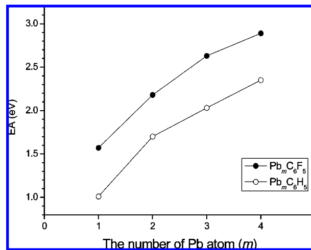
Figure 4. The comparison between the EAs of the Pb_mC_6F_5^- and Pb_mC_6H_5^- complexes.
