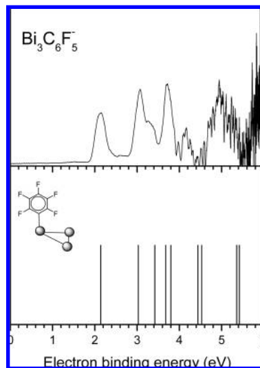
Figure 13. The comparison of PE spectrum of Bi_3C_6F_5^- with the simulated spectrum based on Koopmans' theorem for isomer 3a of Bi_3C_6F_5^- .
