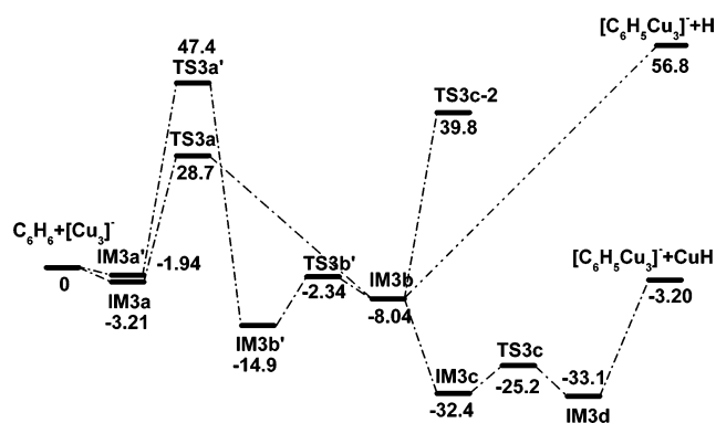
Figure 8. Relative energy profile along the reaction pathway of [\text{C}_6\text{H}_5\text{Cu}_3]^- formation.
